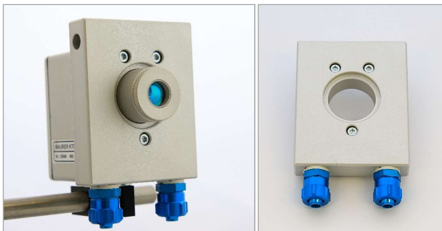
Cooling plate, installed to compact pyrometer and as individual part
